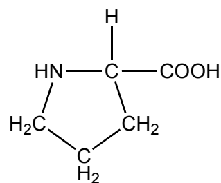
proline
