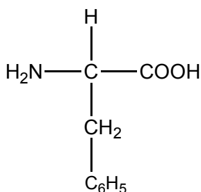
phenylalanine
